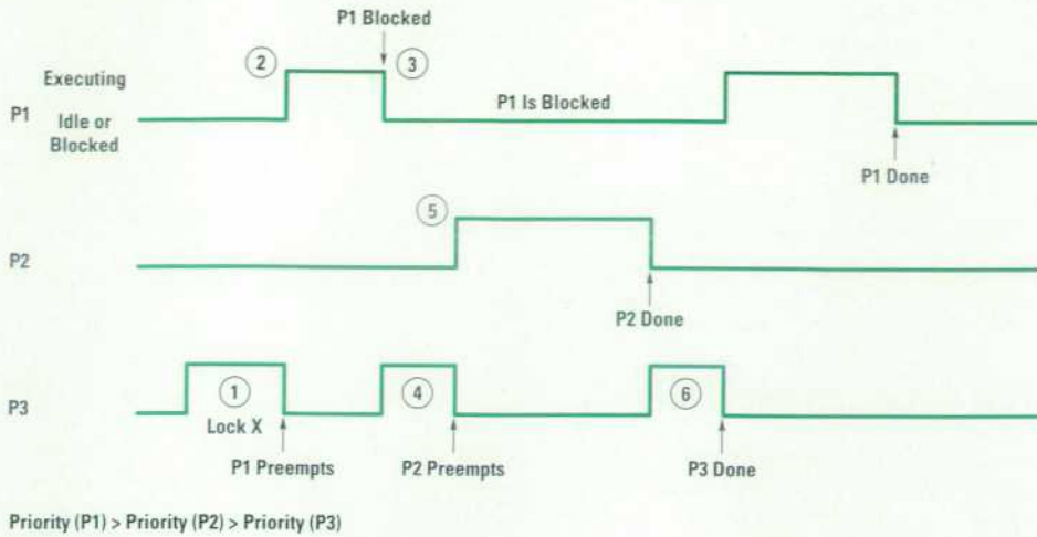
Fig. 7. A time line illustrating priority inversion.
