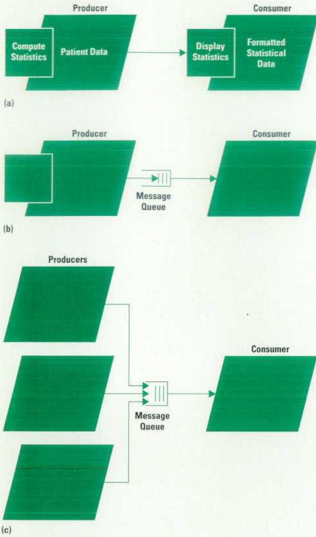
Fig. 6. ADARTS diagrams modeling intertask communication and synchronization. (a) Tightly coupled communication. (b) Loosely coupled communication. (c) Loosely coupled communication with multiple producers.
