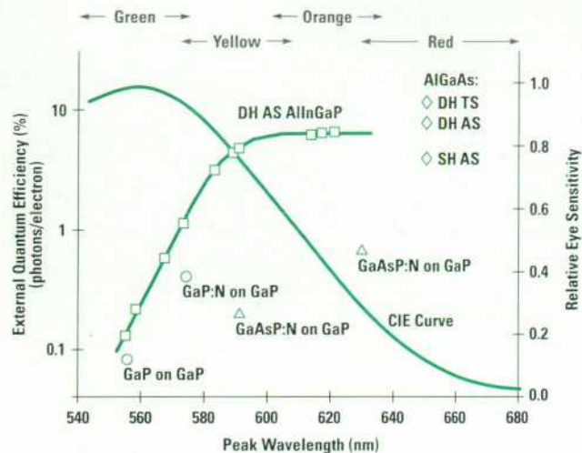
Fig. 5. External quantum efficiency of T-1/4 AlInGaP lamps compared to other technologies. Also shown is the CIE human-eye response curve.
