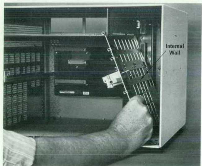
Fig. 3. Gaining access to the Model 747i backplane by removing the internal wall.
