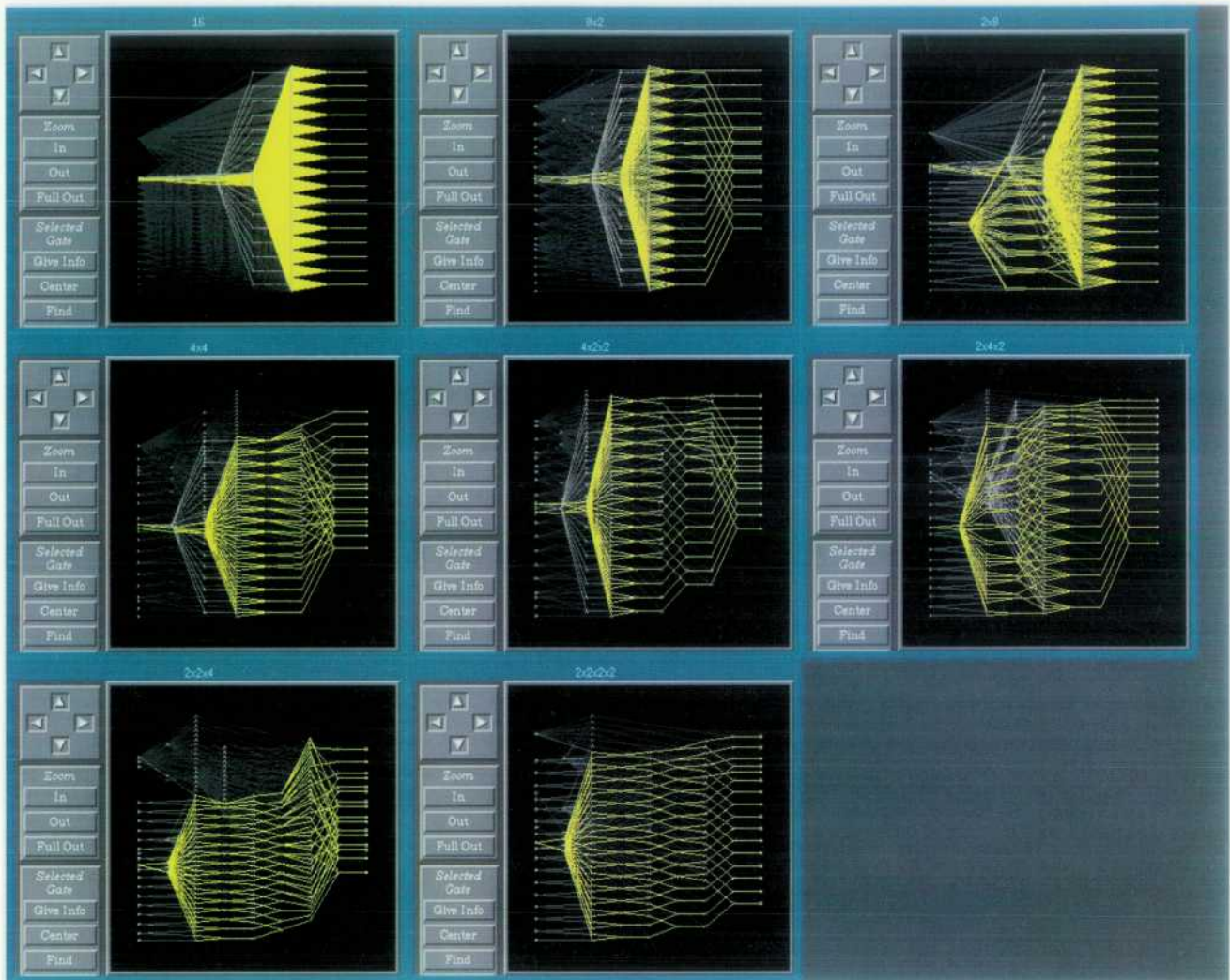
Fig. 4. All eight possible organizations for a 16-bit unidirectional shifter are shown in this topology graph mosaic. The organizations derive from the factorizations of 16, the bit width. The factorization (2 4 2) results in a shifter composed of a level of 2-to-1 multiplexers followed by a level of 4-to-1 multiplexers and finally followed by a level of 2-to-1 multiplexers.
