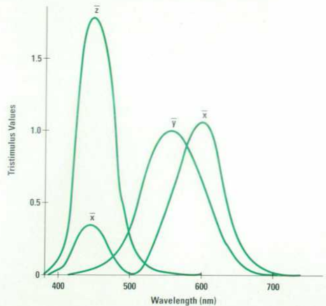
Fig. 1. CIE standard observer color matching curves.
