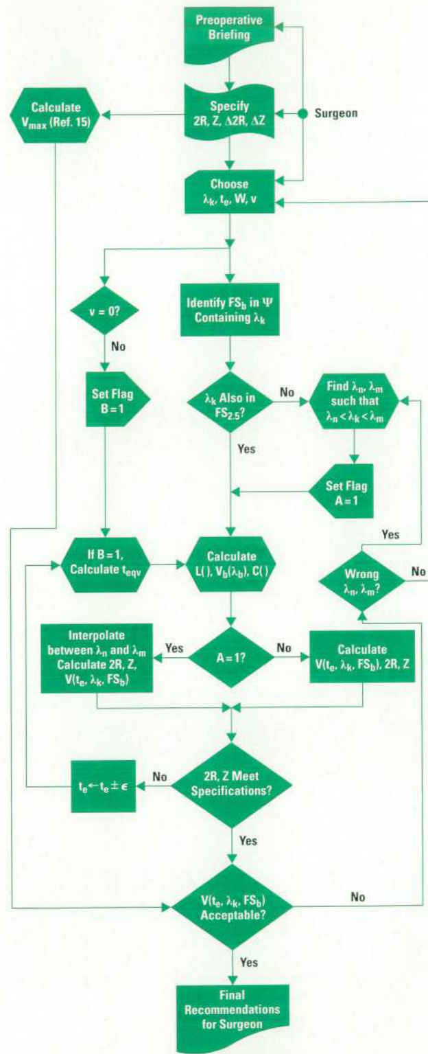
Fig. 4. Flowchart of the LCA algorithm.
